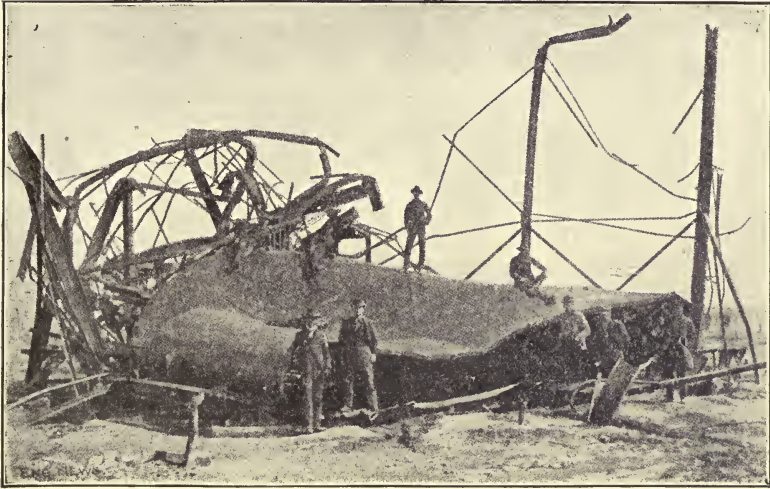
FIG. 1.—View of Wrecked Water Tank-tower at Abilene, Texas.
